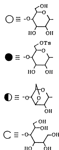
Scheme 1. Structure determination of 6 A ,6 X ,6 Y -trisulfonates 1a-e.
